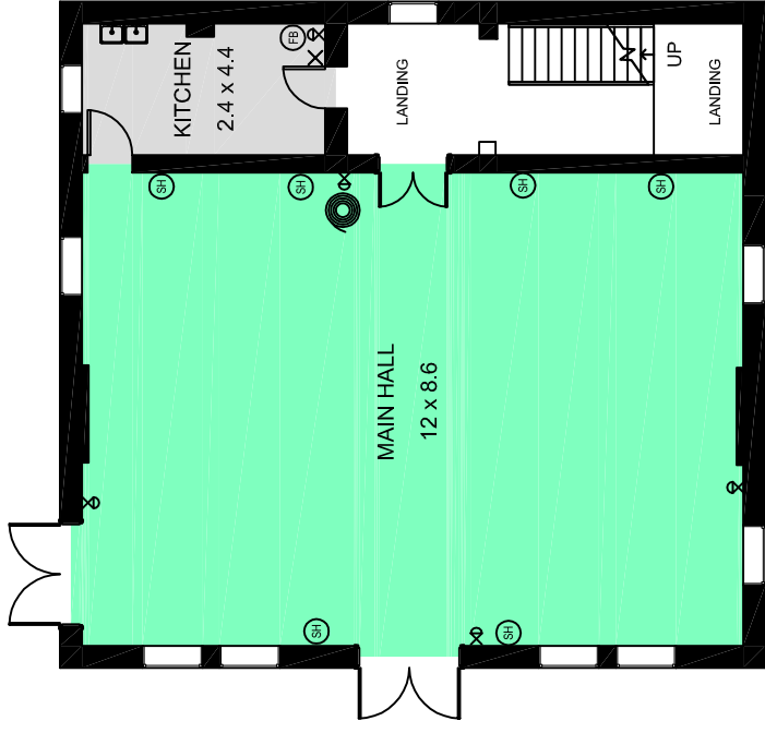
FIRST FLOOR PLAN "ANNANDALE NEIGHBOURHOOD CENTRE"
